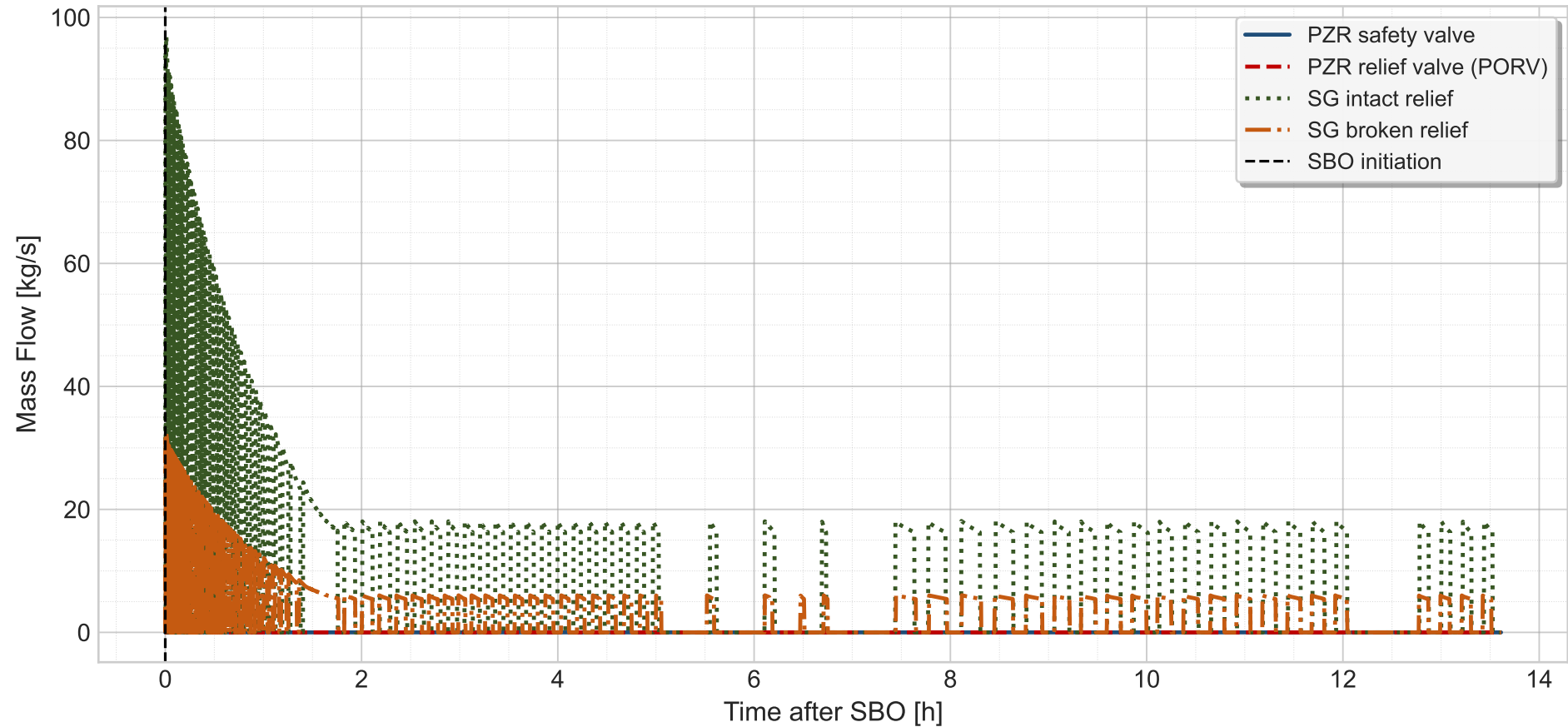
Base Case - Relief and Safety Valves
